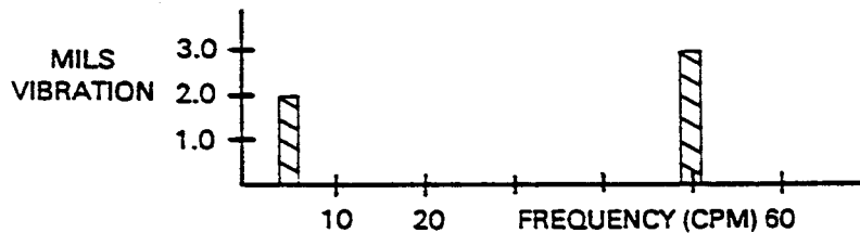
Figure 21 A simple vibration signature.
